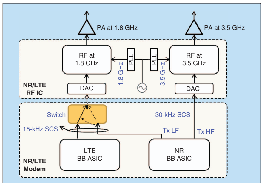
FIGURE 8 The joint NR/LTE UE architecture [14]. PA: power amplifier; DAC: digital-to-analog converter; IC: integrated circuit; PLL: phase-locked loop; HF: high frequency; LF: low frequency; BB ASIC: base-band application-specific integrated circuit; RF: radio frequency.
