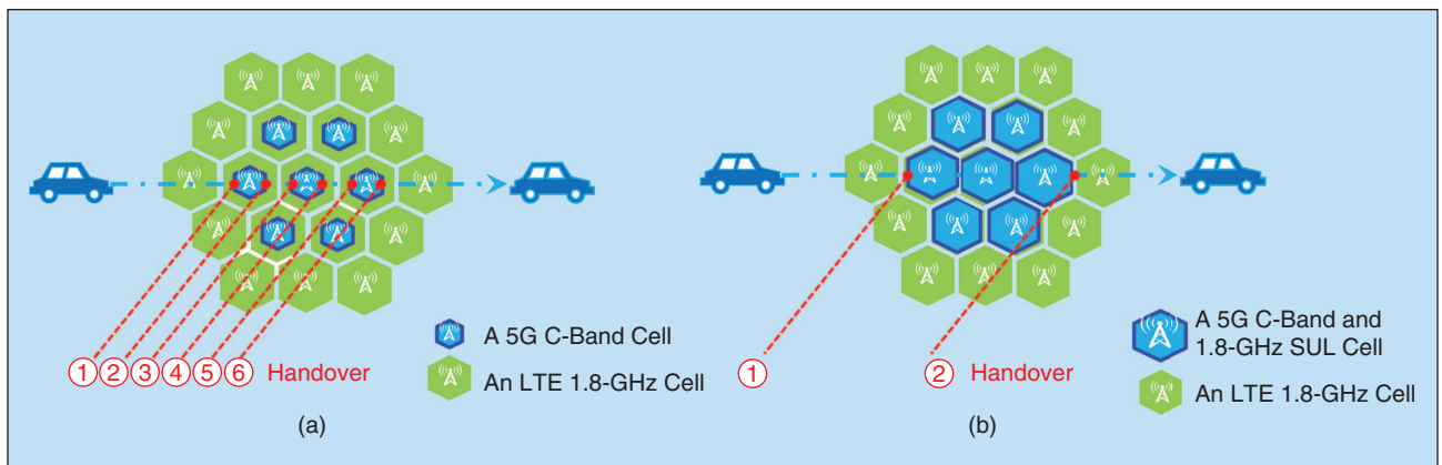
FIGURE 6 The seamless coverages by cosite NR/LTE deployments. (a) The UL over only higher-frequency bands and (b) the UL over both C- and lower-frequency bands.
