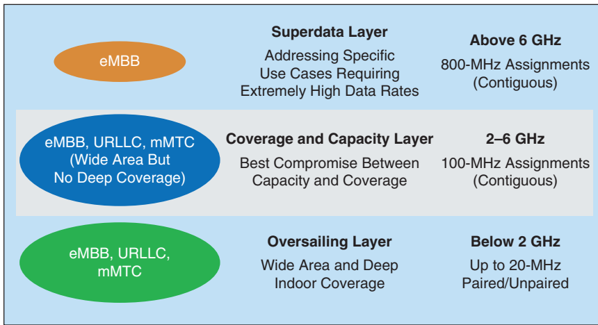
FIGURE 1 A multilayer approach for 5G scenarios.
