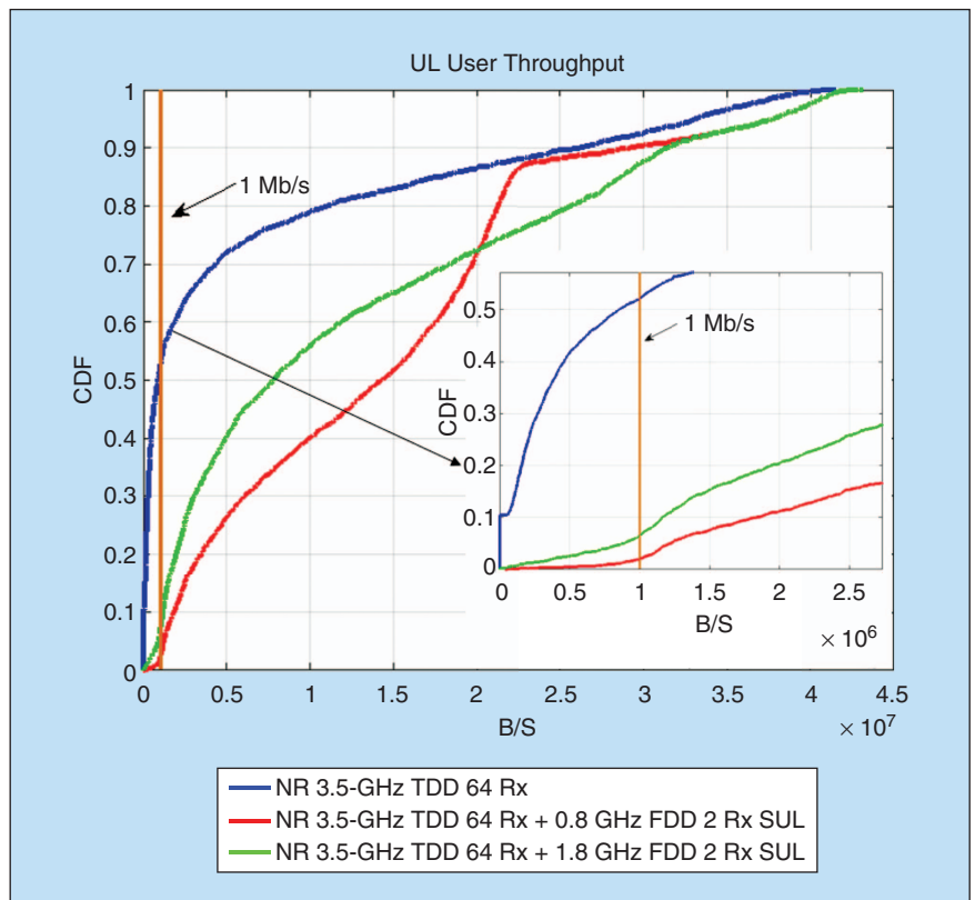
FIGURE 4 The UL user-throughput comparison. CDF: cumulative distribution function.
